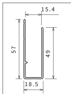
compensation R-2A-2P-2PH-A-AH
